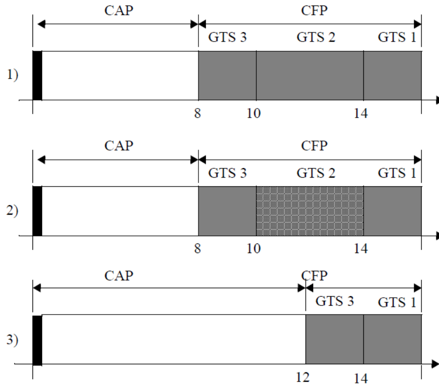
Figure 33 — CFP defragmentation on GTS deallocations
