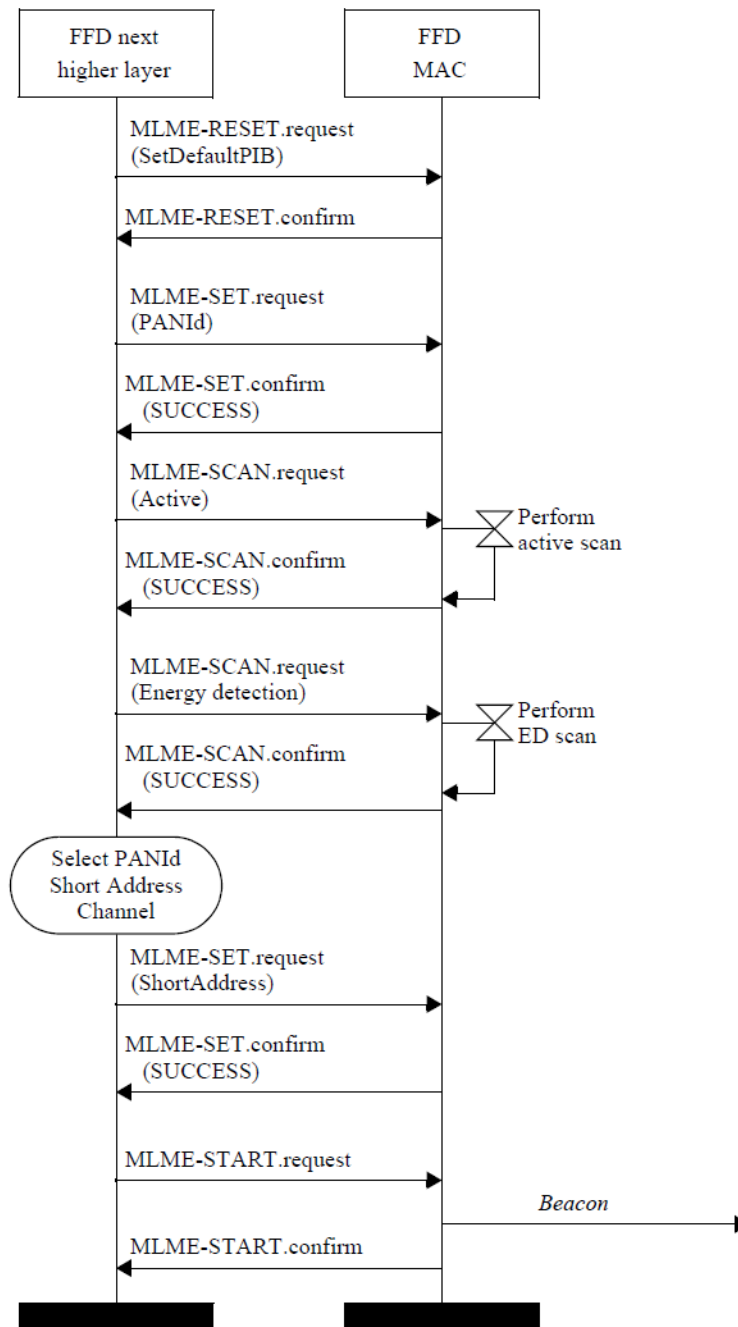
Figure 16 — PAN start message sequence chart—PAN coordinator
