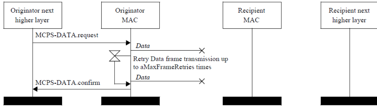
Figure 28 — Lost data frame message sequence
