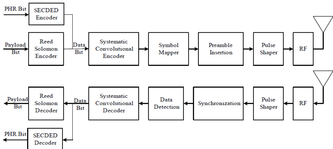
Figure 83 — Figure 83—UWB PHY signal flow
