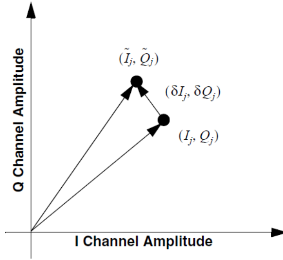
Figure 65 — Error-vector calculation
