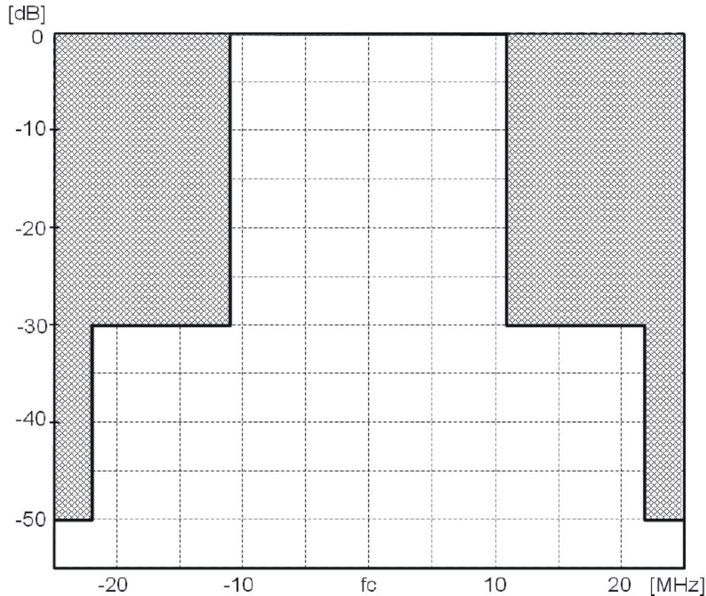
Figure 82 — Transmit PSD mask
