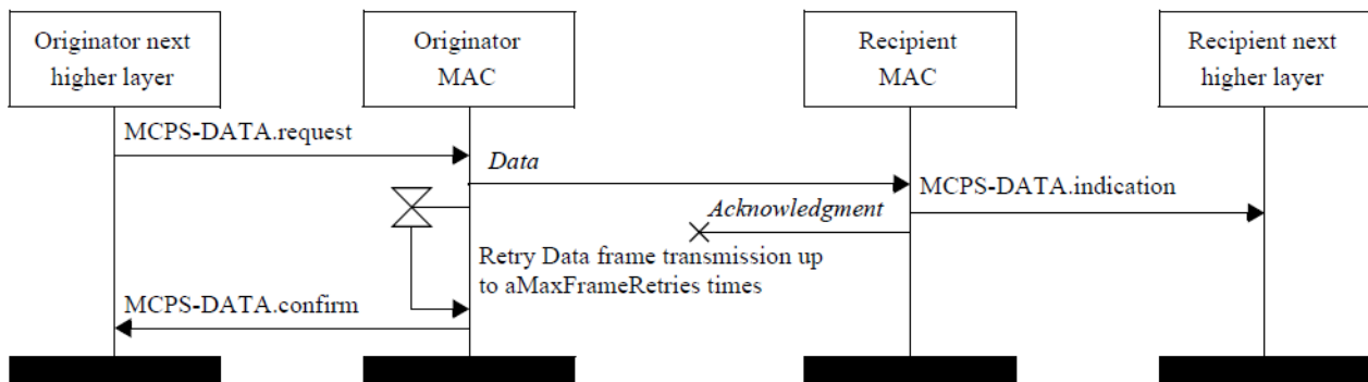
Figure 29 — Lost acknowledgment message sequence
