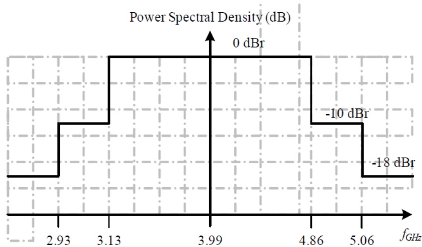
Figure 96 — Transmit spectrum mask for band 4
