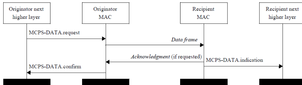
Figure 27 — Successful data transmission sequence
