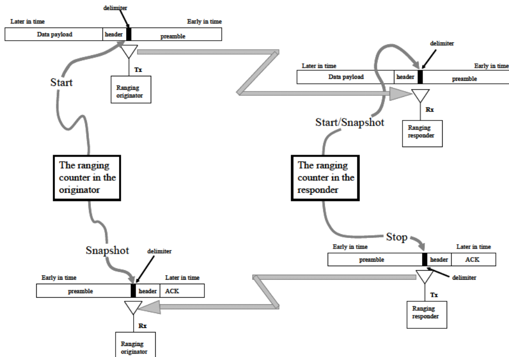
Figure E.1 — The complete two-way ranging technique
