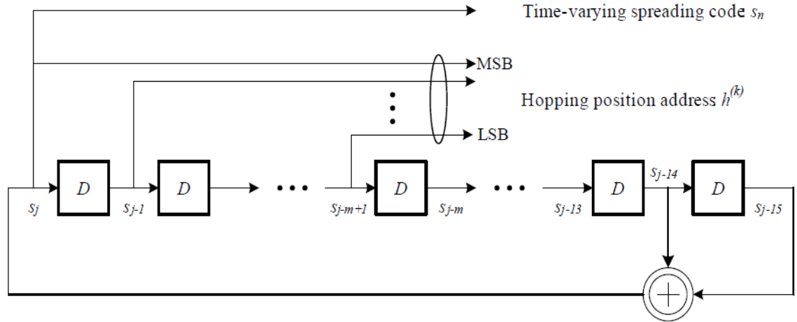
Figure 91 — LFSR implementation of the scrambler
