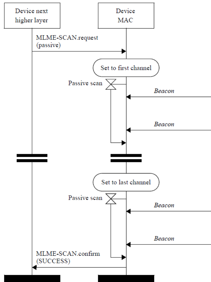
Figure 13 — Passive scan message sequence chart
