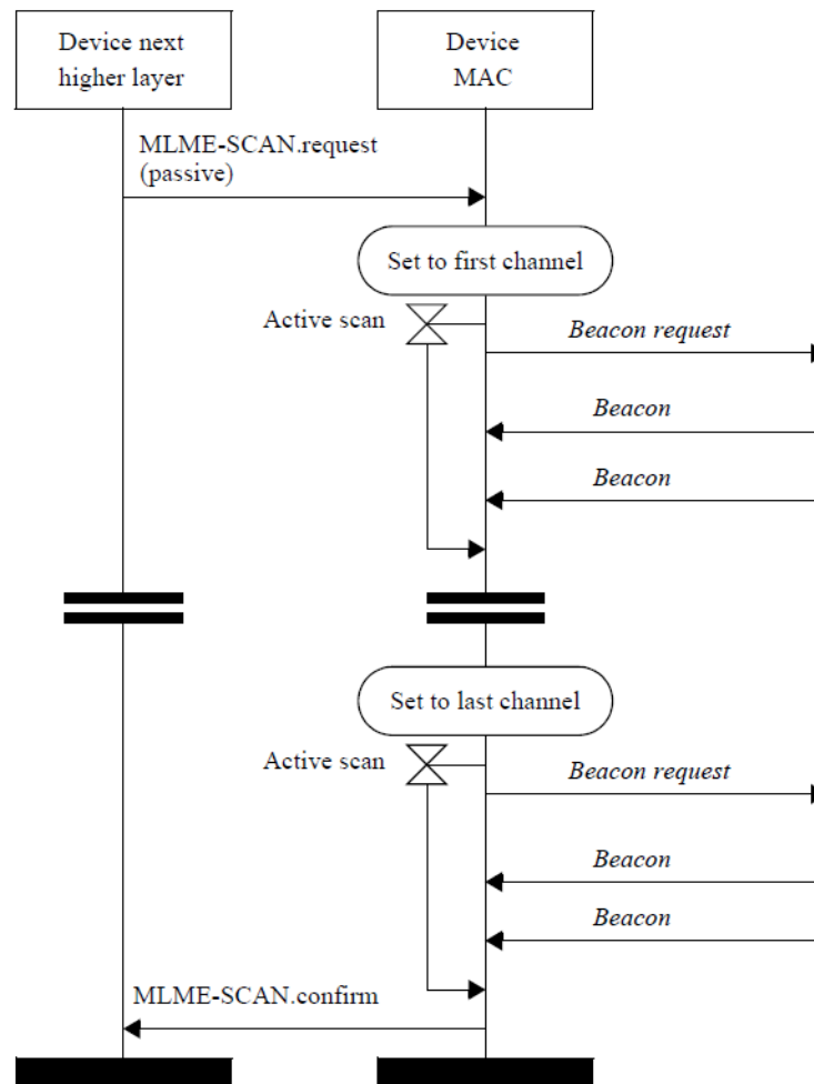
Figure 12 — Active scan message sequence chart
