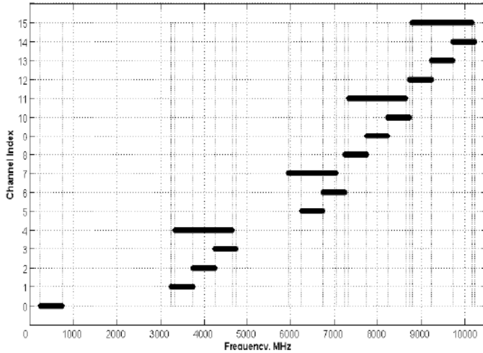
Figure 94 — UWB PHY band plan
