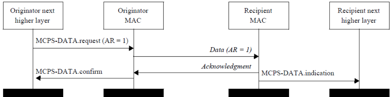
Figure 26 — Successful data transmission with an acknowledgment
