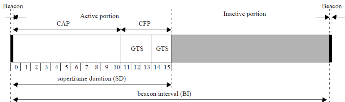
Figure 8 — An example of the superframe structure
