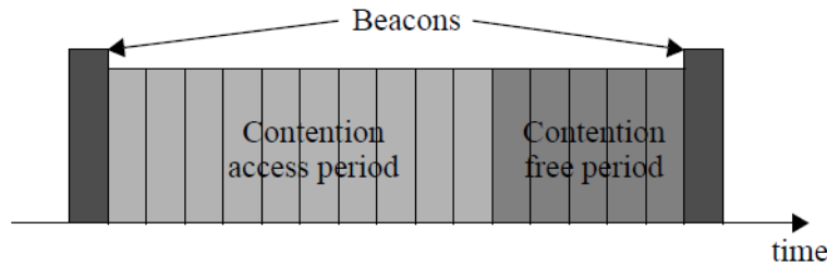
Figure 5 — Structure of the active periods with GTSS
