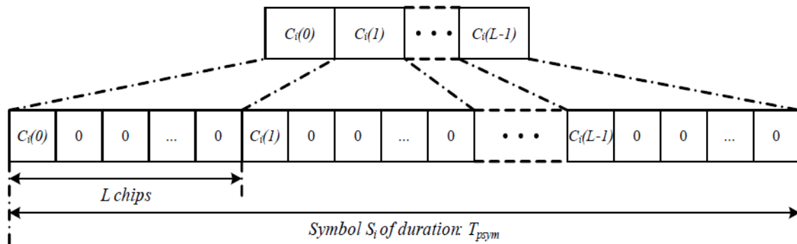
Figure 87 — Construction of symbol S_i from code C_i
