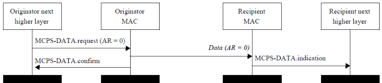
Figure 25 — Successful data transmission without an acknowledgment
