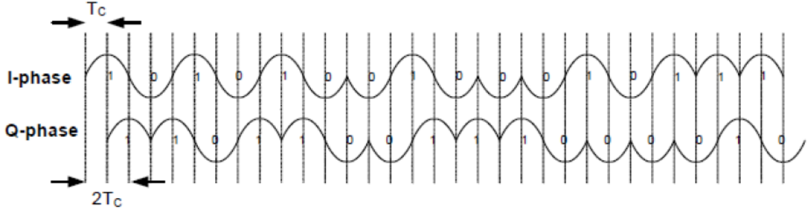
Figure 71 — Sample baseband chip sequences with pulse shaping
