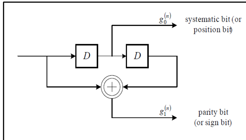
Figure 93 — Systematic convolutional encoder
