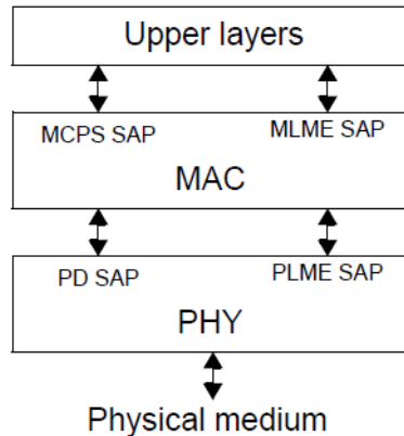
Figure 3 — LR-WPAN device architecture
