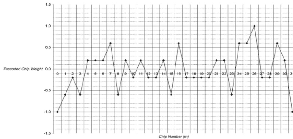
Figure 75 — Precoded PSSS symbol p''(m)
