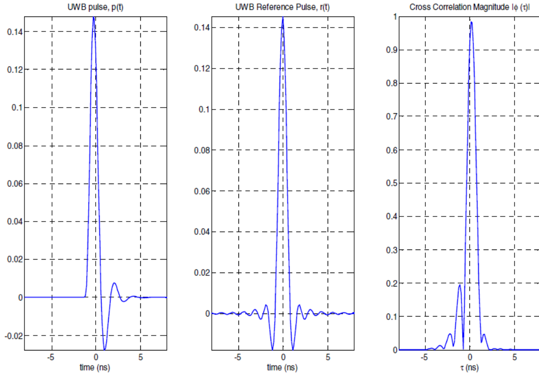
Figure 95 — Compliant pulse example
