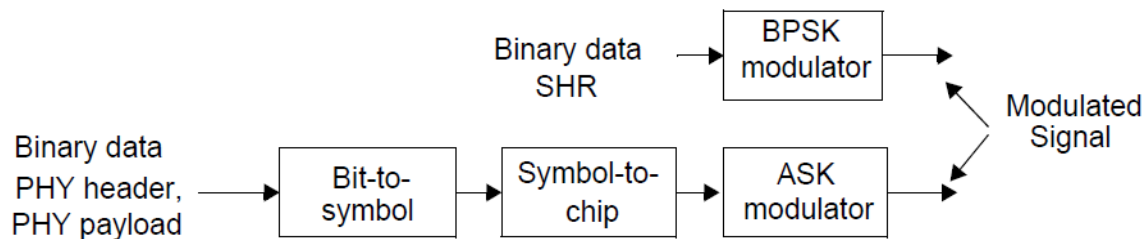
Figure 73 — Modulation and spreading functions
