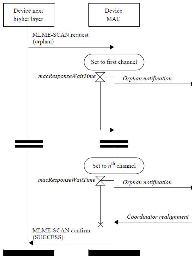
Figure 14 — Orphaned device realignment message sequence chart
