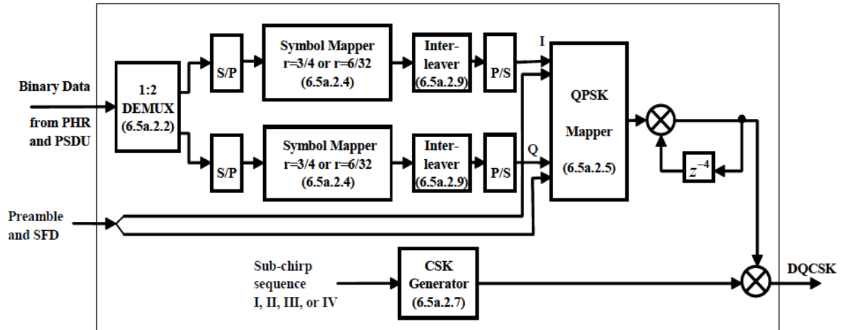
Figure 78 — Differential bi-orthogonal quaternary-chirp-shift-keying modulator and spreading ( r = 3/4 for 8-ary 1 Mb/s, r = 3/16 for 64-ary 250 kb/s)
