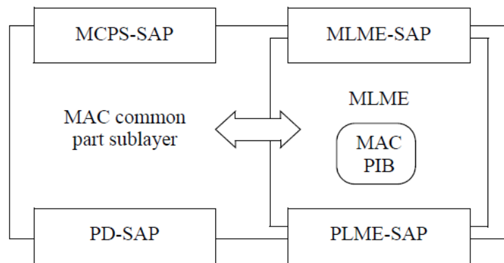
Figure 60 — MAC sublayer reference model
