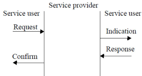
Figure 7 — Service primitives
