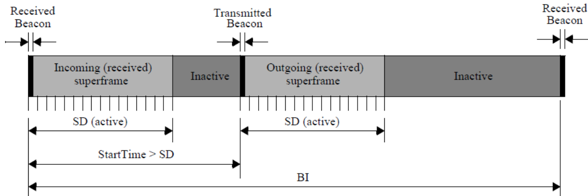
Figure 9 — The relationship between incoming and outgoing beacons
