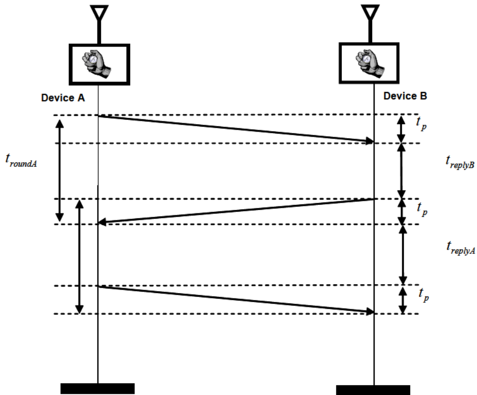
Figure E.9 — Exchange of message in SDS-TWR
