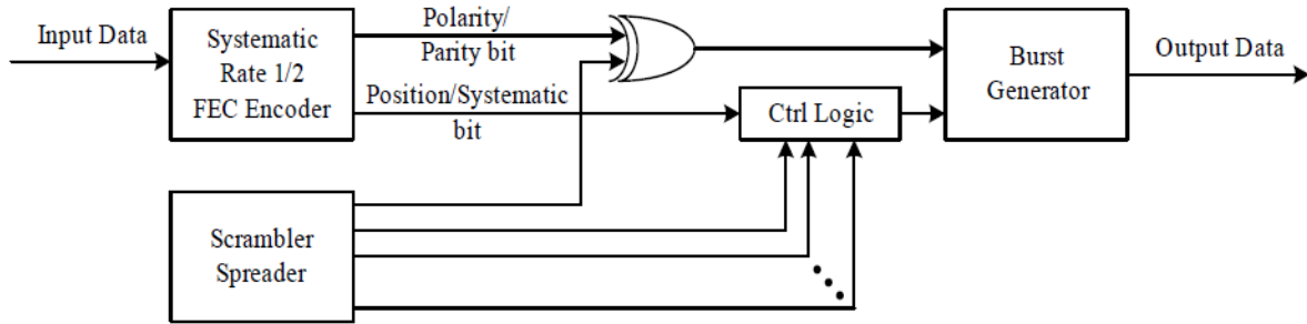
Figure 90 — Reference symbol modulator
