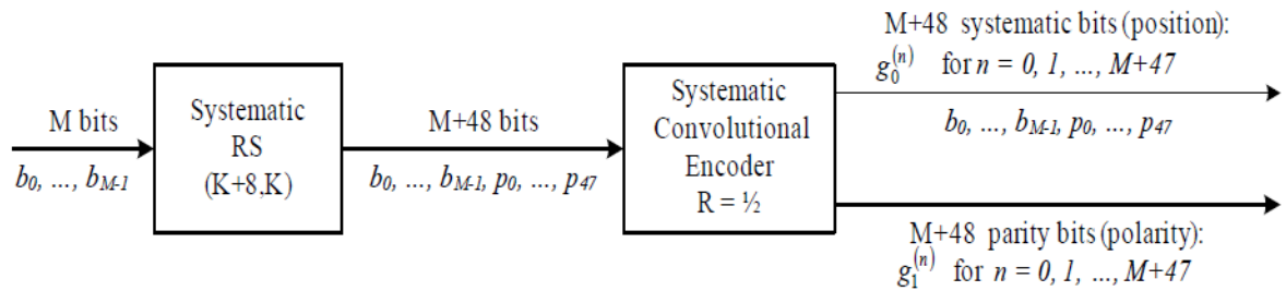
Figure 92 — FEC encoding process
