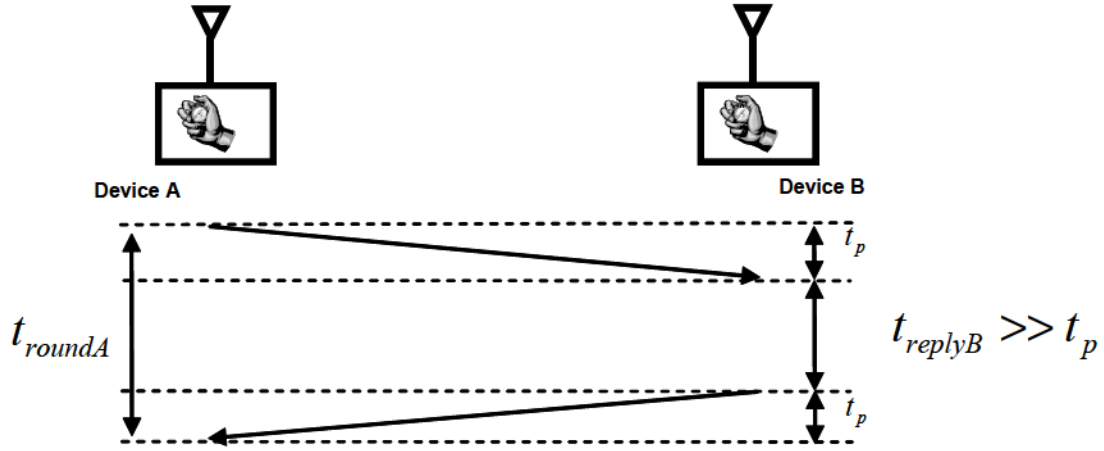
Figure E.8 — Exchange of message in two-way ranging
