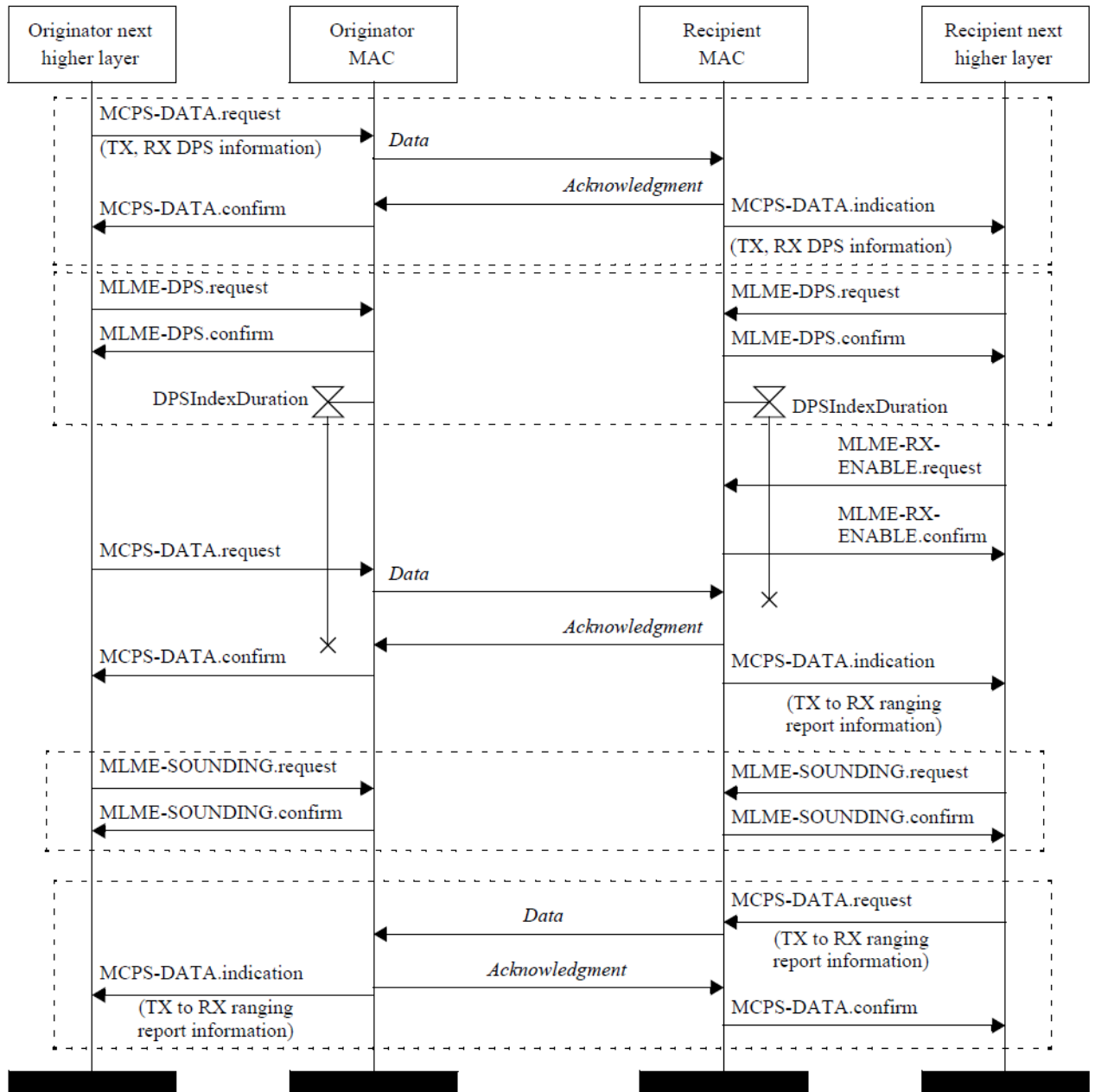
Figure 34 — A message sequence for ranging
