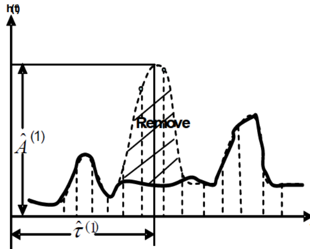
Figure E.6 — Leading-edge detection in NLOS conditions
