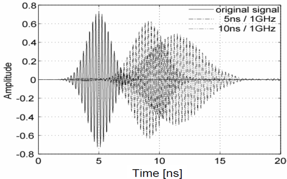
Figure 98 — Examples of CS pulses
