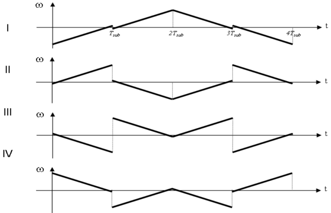
Figure 79 — Four different combinations of subchirps
