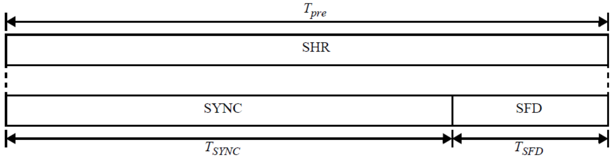
Figure 86 — SHR preamble structure
