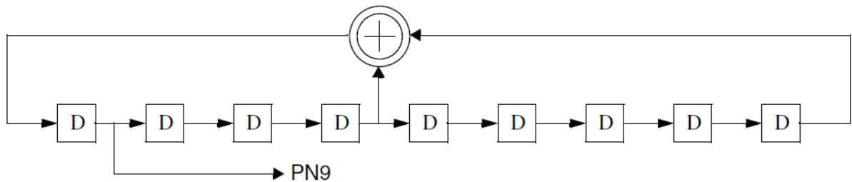
Figure 102 — Schematic of the PN generator
