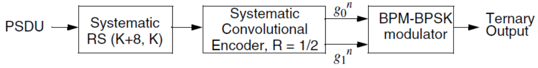
Figure 89 — Data field encoding process
