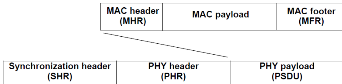
Figure 6 — Schematic view of the PPDU
