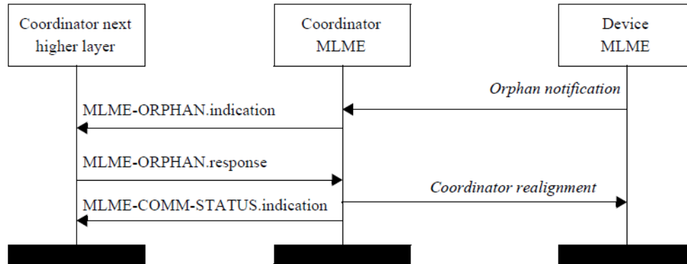
Figure 15 — Message sequence chart for orphan notification
