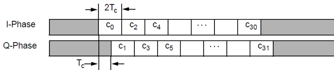
Figure 70 — O-QPSK chip offsets
