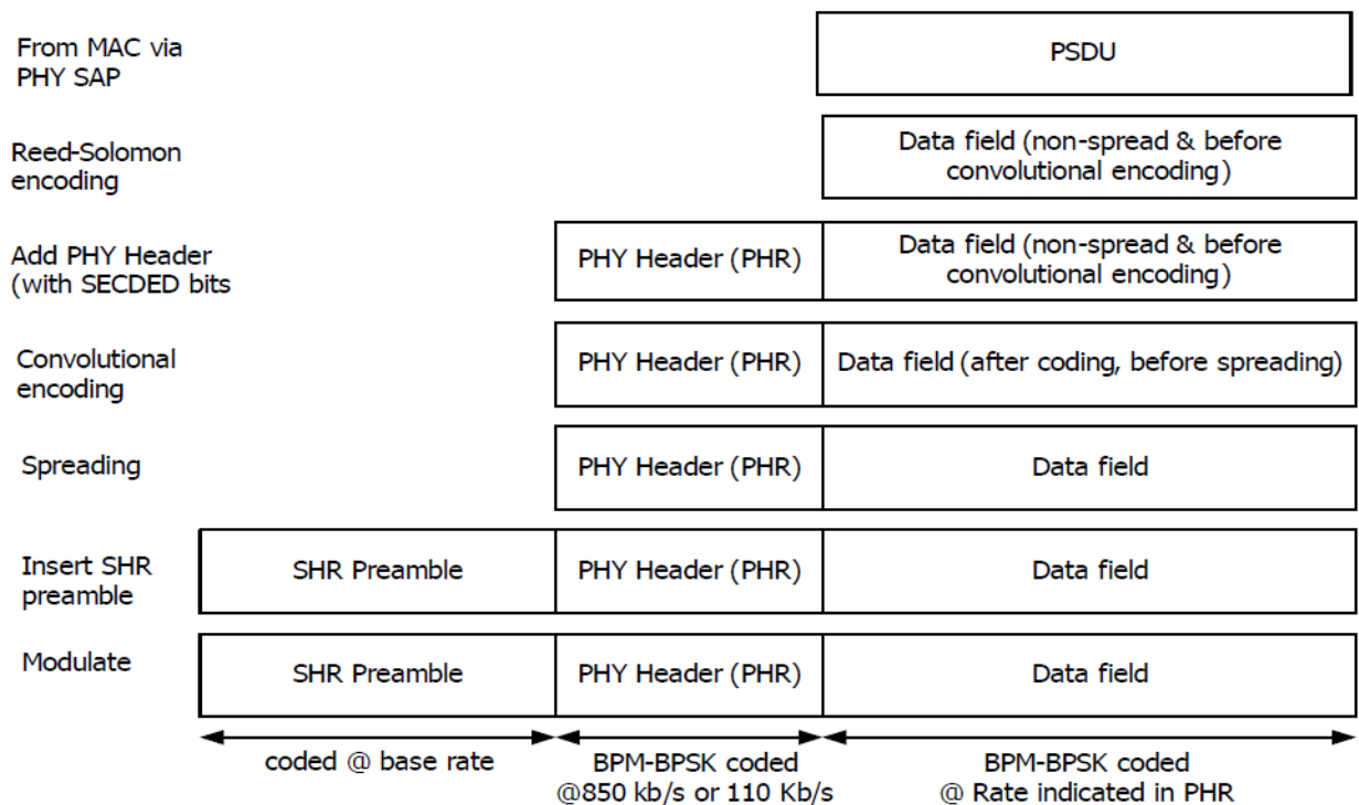
Figure 84 — UWB PPDU encoding process
