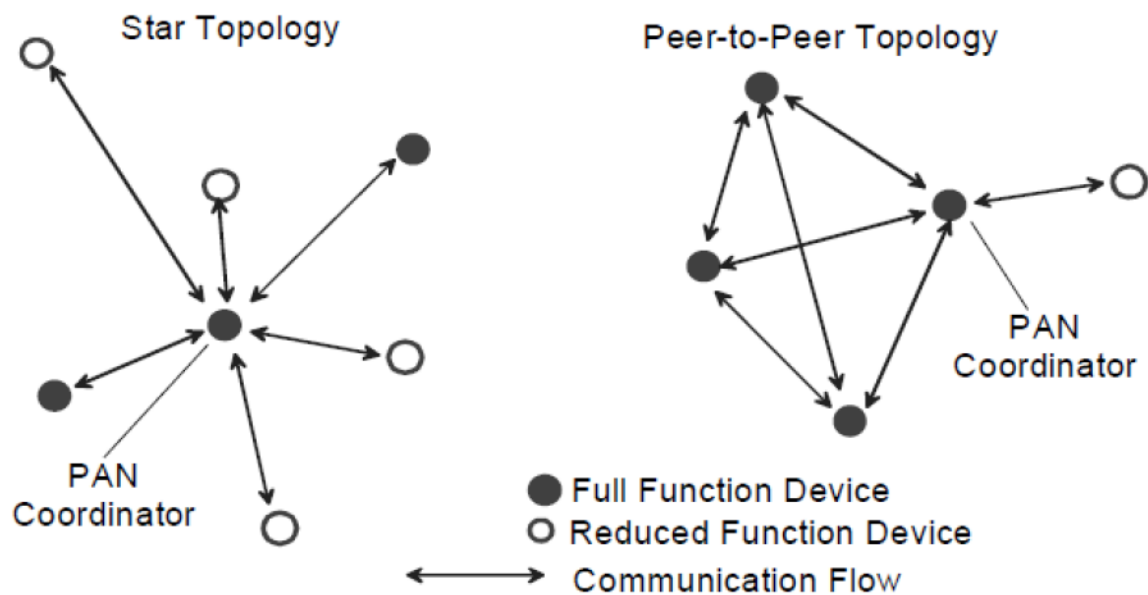
Figure 1 — Star and peer-to-peer topology examples
